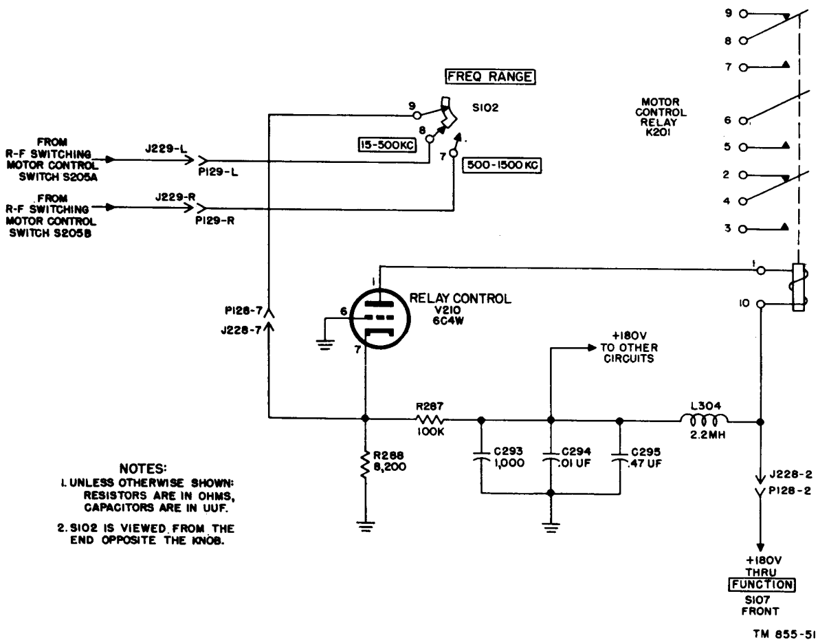
Figure 39. Relay control, schematic diagram.
