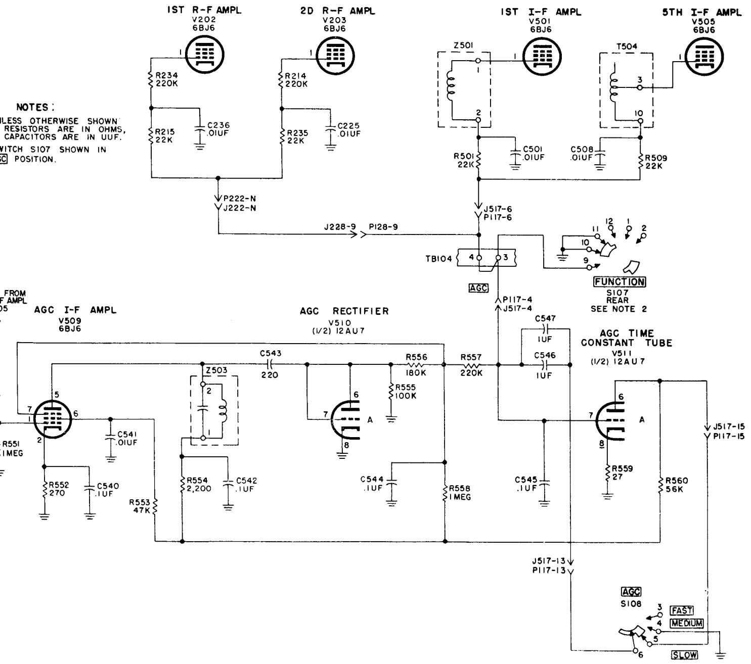
Figure 86. Age voltage distribution.
