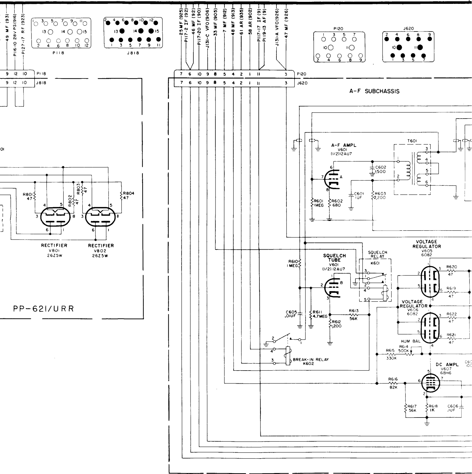
Figure 88. Subchassis and interconnection diagram—Continued.
