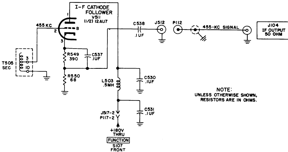
Figure 30. I-f. cathode follower, schematic diagram.
