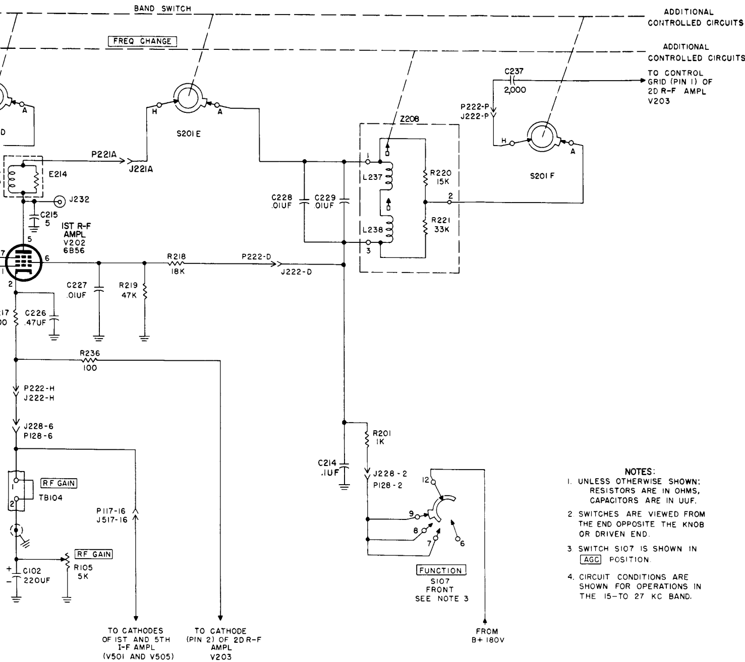
Unit and first rf amplifier, schematic diagram.
