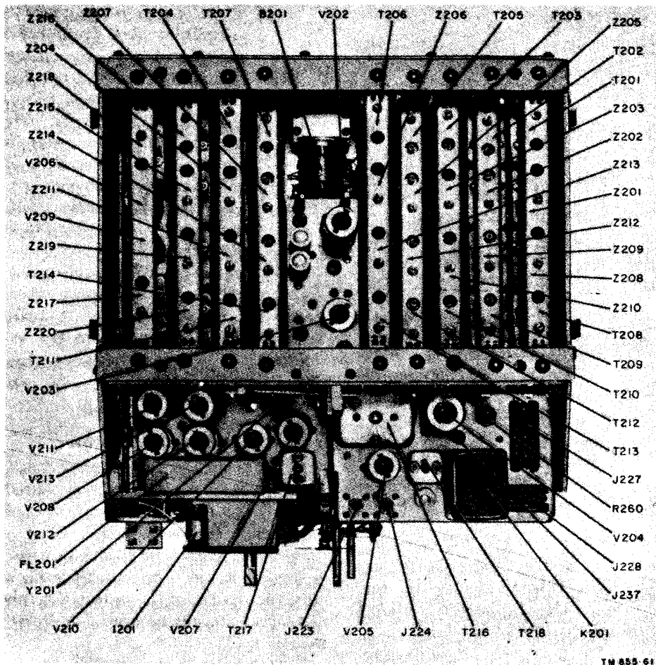
Figure 49. Rf subchassis, top view.
