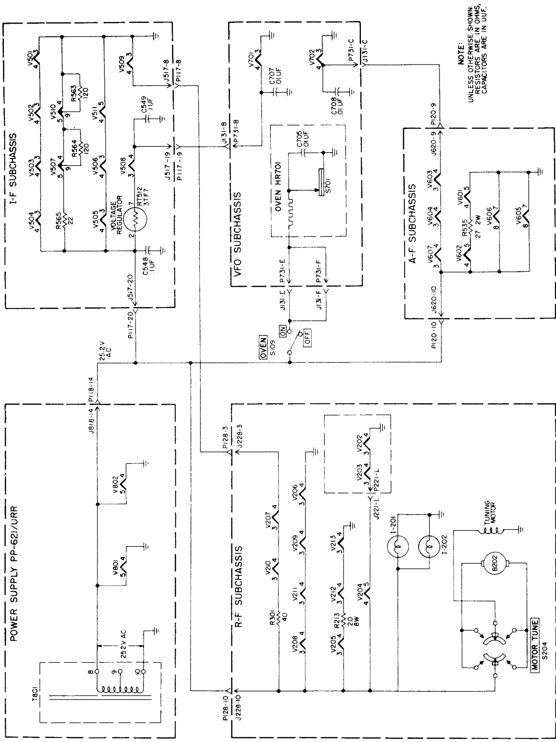
Figure 37. Filament, oven heater, and tuning motor circuits, schematic diagram.
