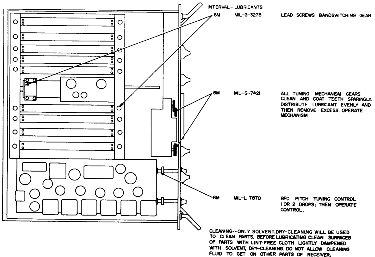
Figure 73. Lubrication of tuning mechanism, slug racks, and band-switching motor.
