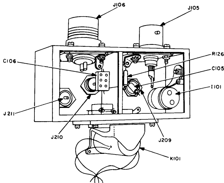
Figure 72. Antenna box, interior view.
