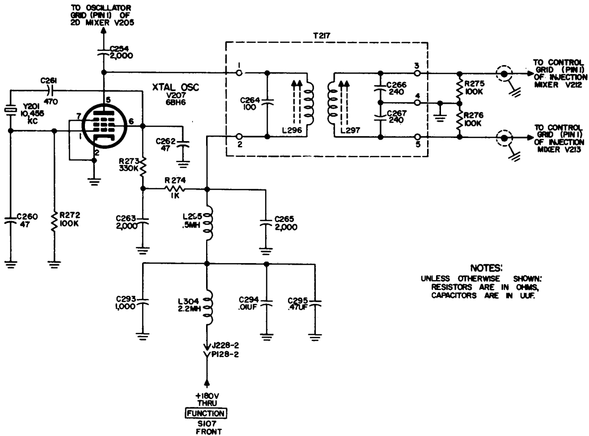
Figure 17. Crystal oscillator, schematic diagram.
