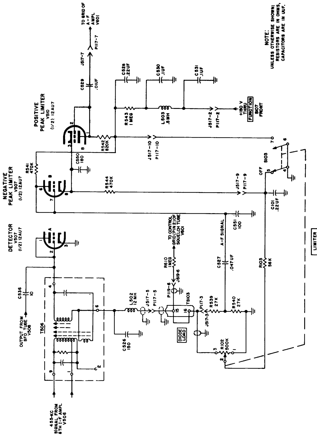
Figure 26. Detector and limiter circuits, schematic diagram.
