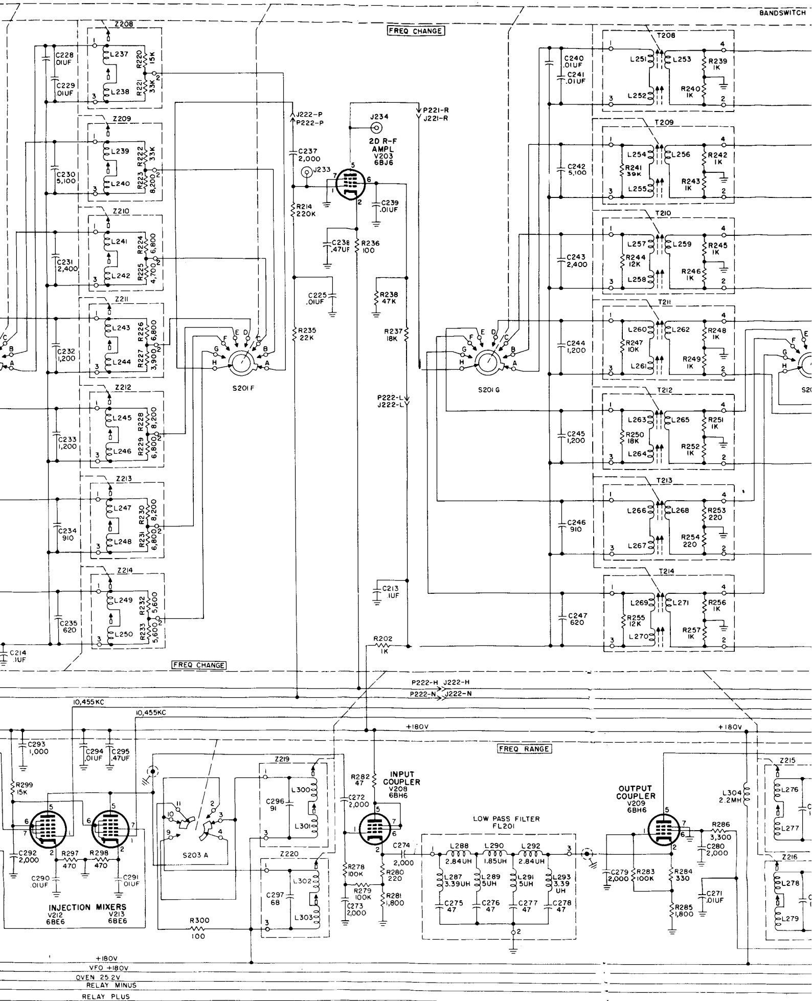
Figure 89. Radio Receiver R-389/URR, schematic diagram.
