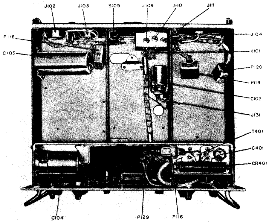
Figure 65. Front panel and main frame, bottom view.
