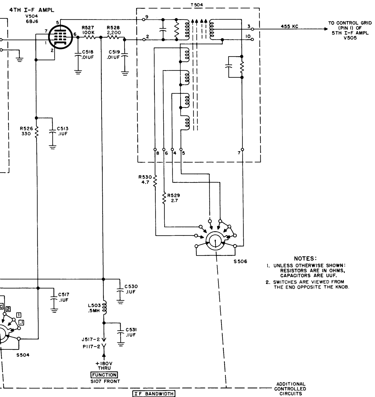
Third and fourth if. amplifiers, schematic diagram.
