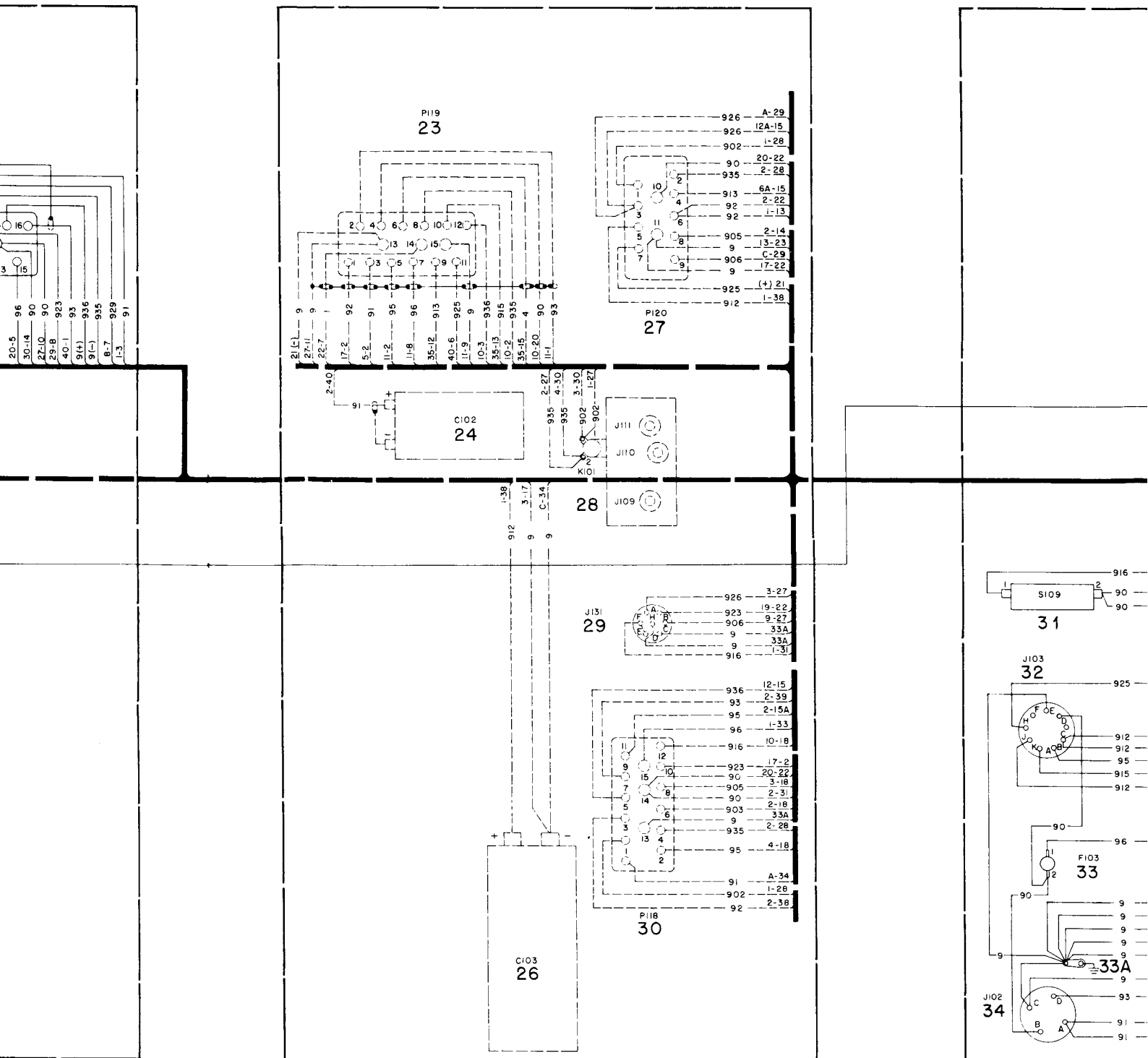
Figure 90. Wiring diagram.
