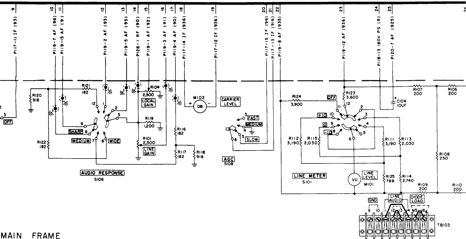
Figure 88. Subchassis and interconnection diagram.
