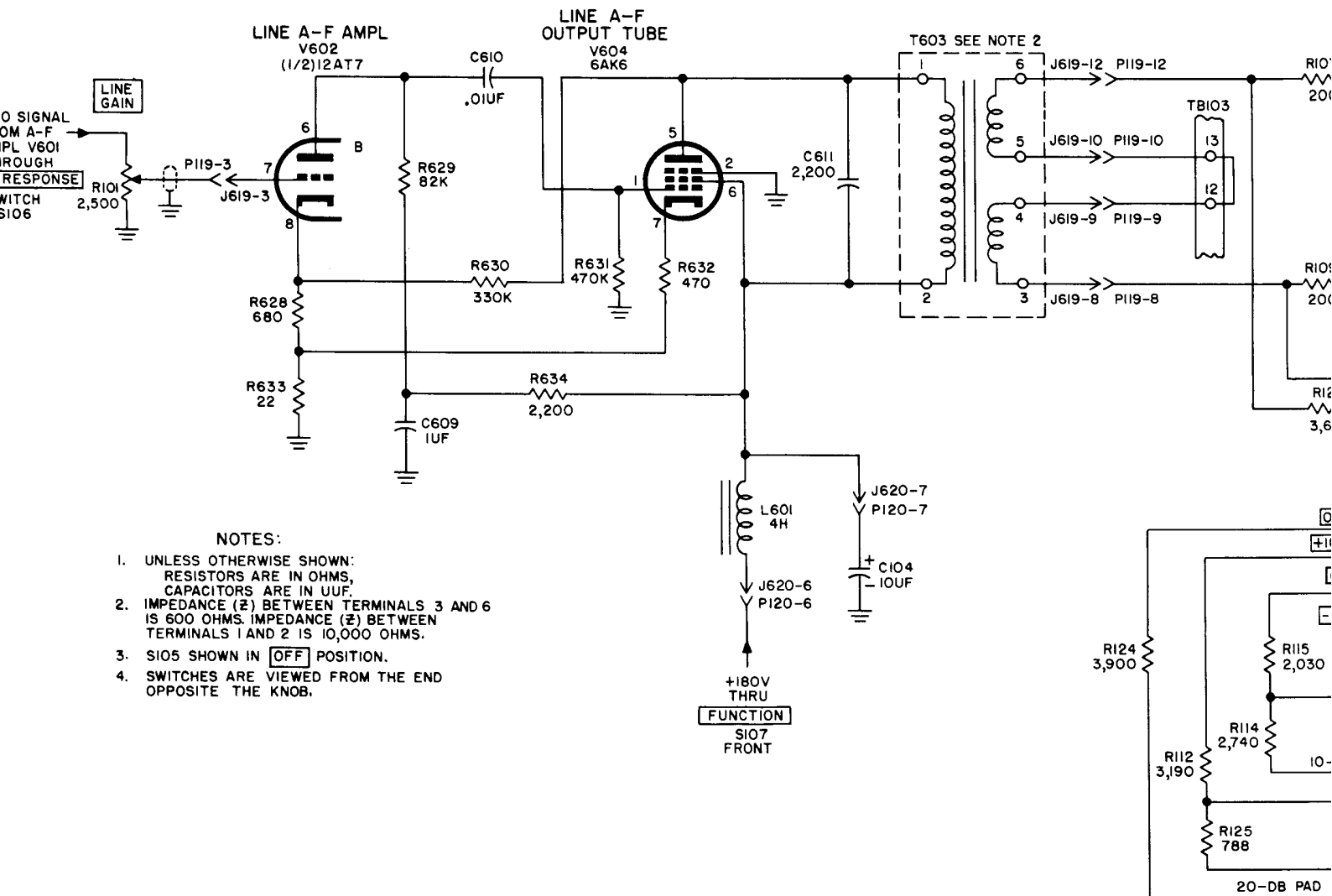
Figure 33. Line audio channel, schematic diagram.
