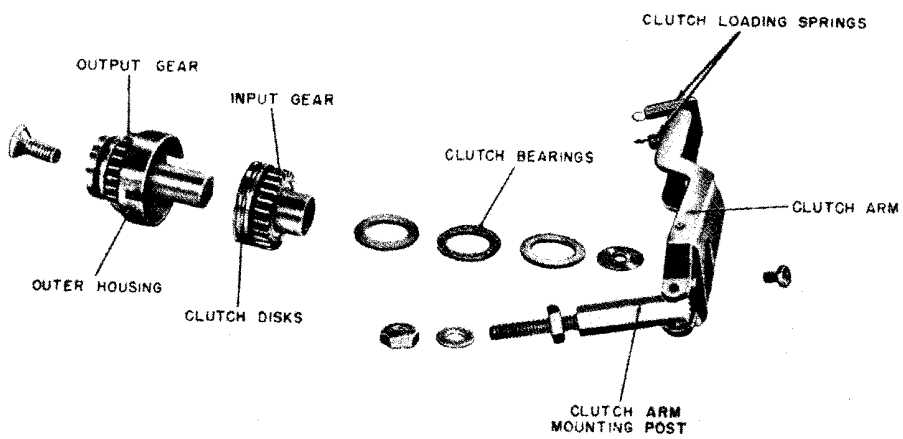
Figure 76. Disk clutch assembly, exploded view.
