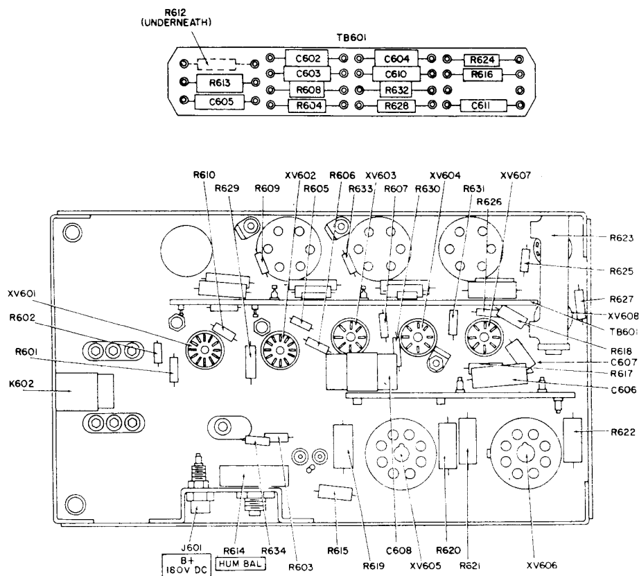
Figure 61. Af subchassis, bottom view.
