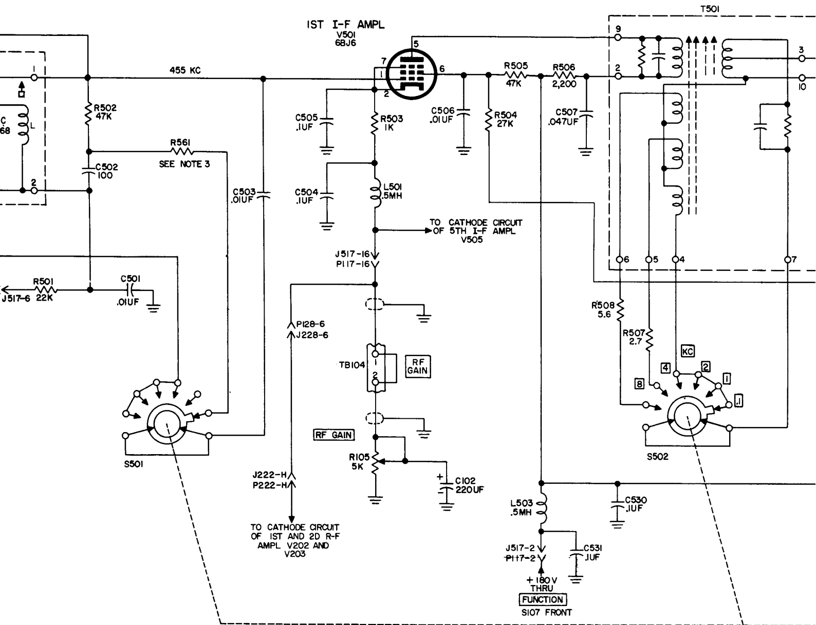
Figure 23. Crystal filter and first and second i-f. amplifiers, schematic diagram.
