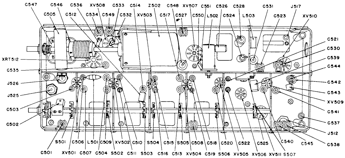
Figure 56. 1F subchassis, bottom view, showing sockets.
