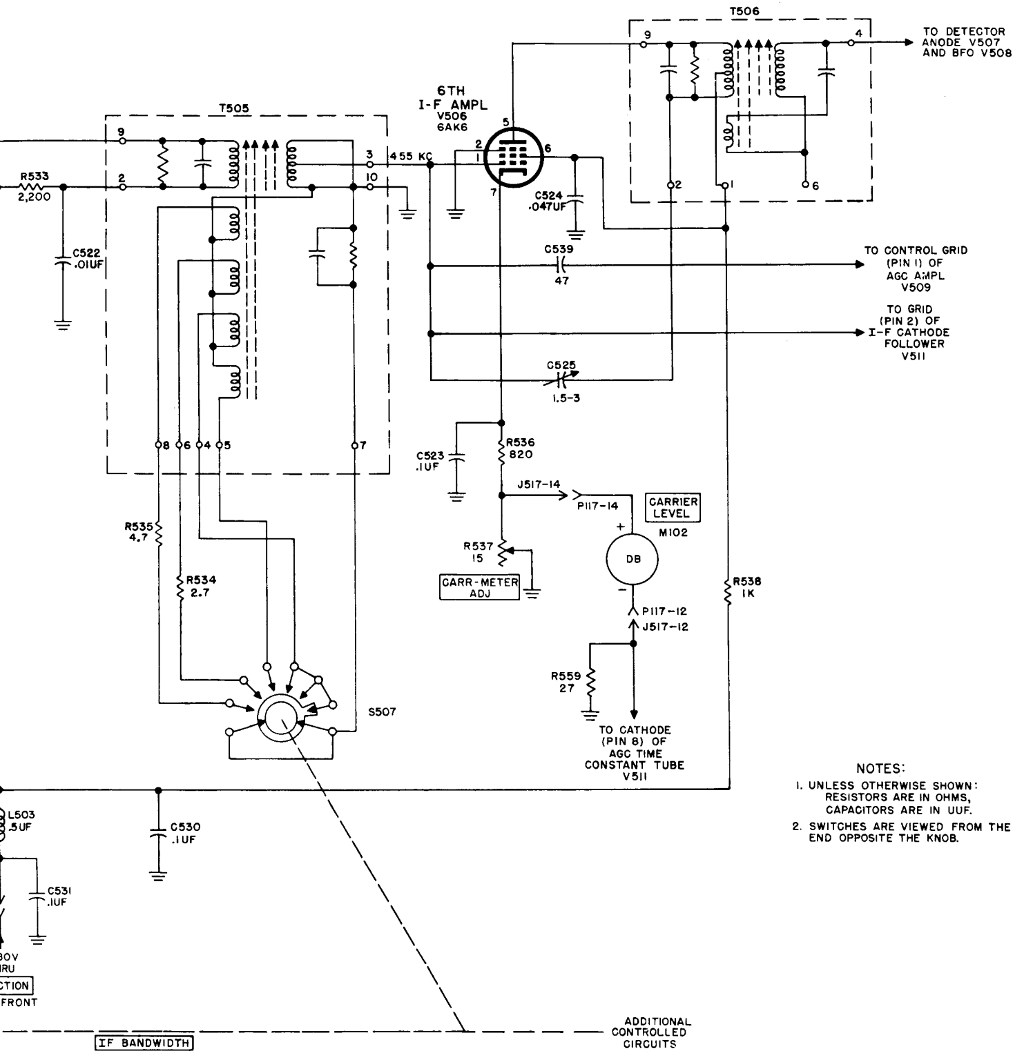
and sixth if. amplifiers, schematic diagram.
