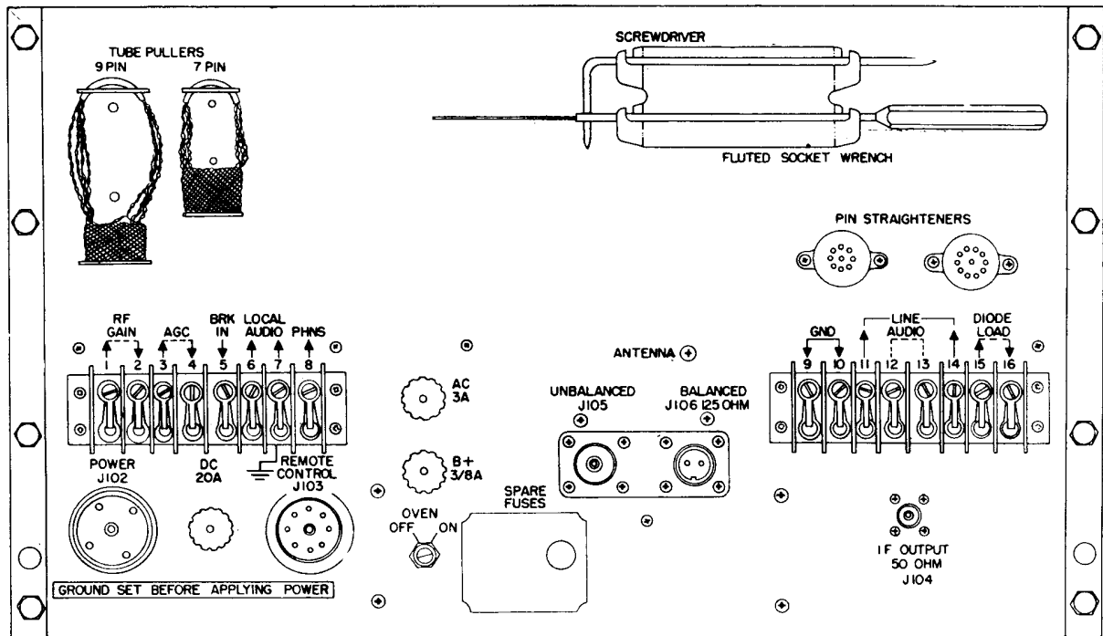
Figure 7. Back panel.
