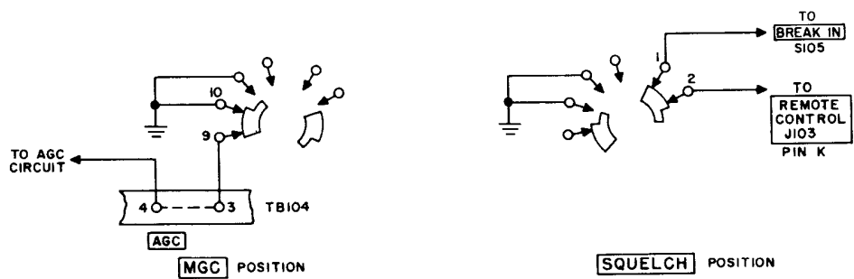
Figure 40. FUNCTION switch, schematic diagram.
