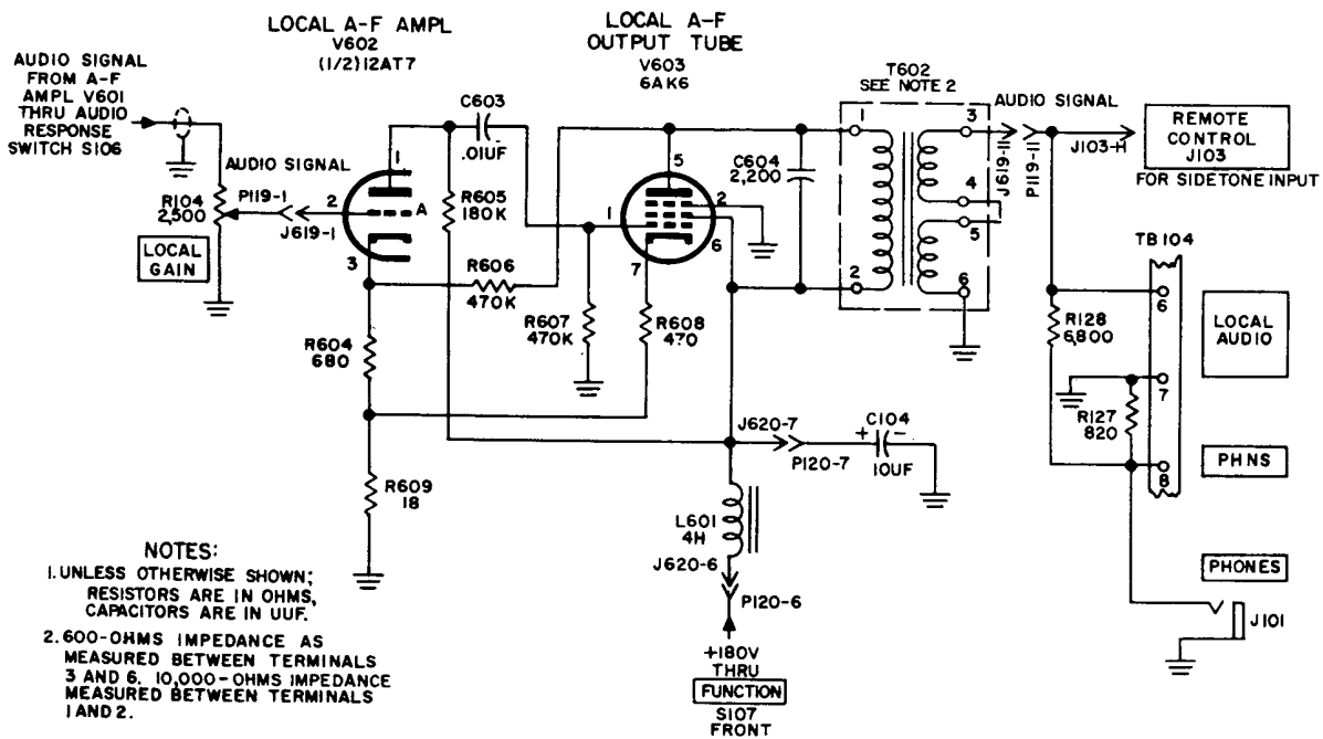
Figure 32. Local audio channel, schematic diagram.
