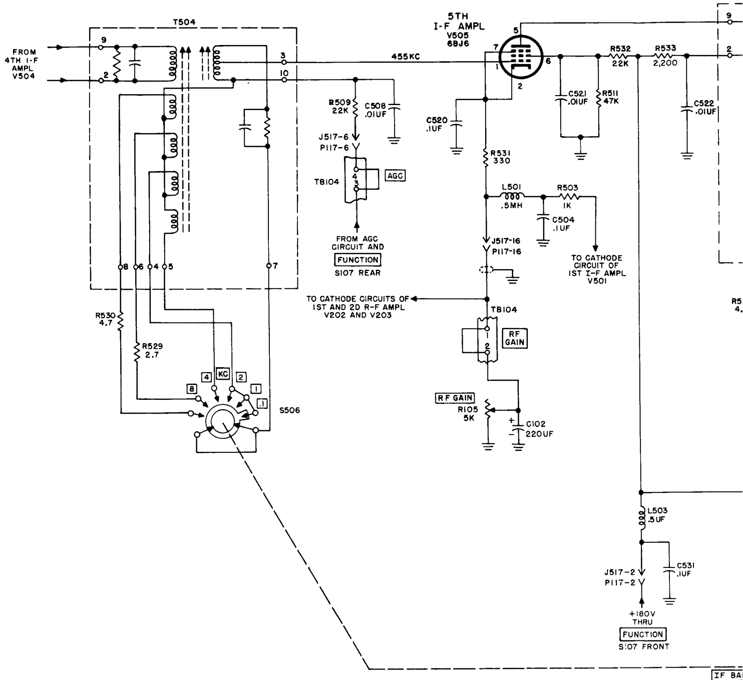
Figure 25. Fifth and sixth if. amplifiers,
