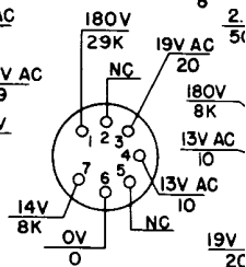
RELAY CONTROL V210 6C4W
