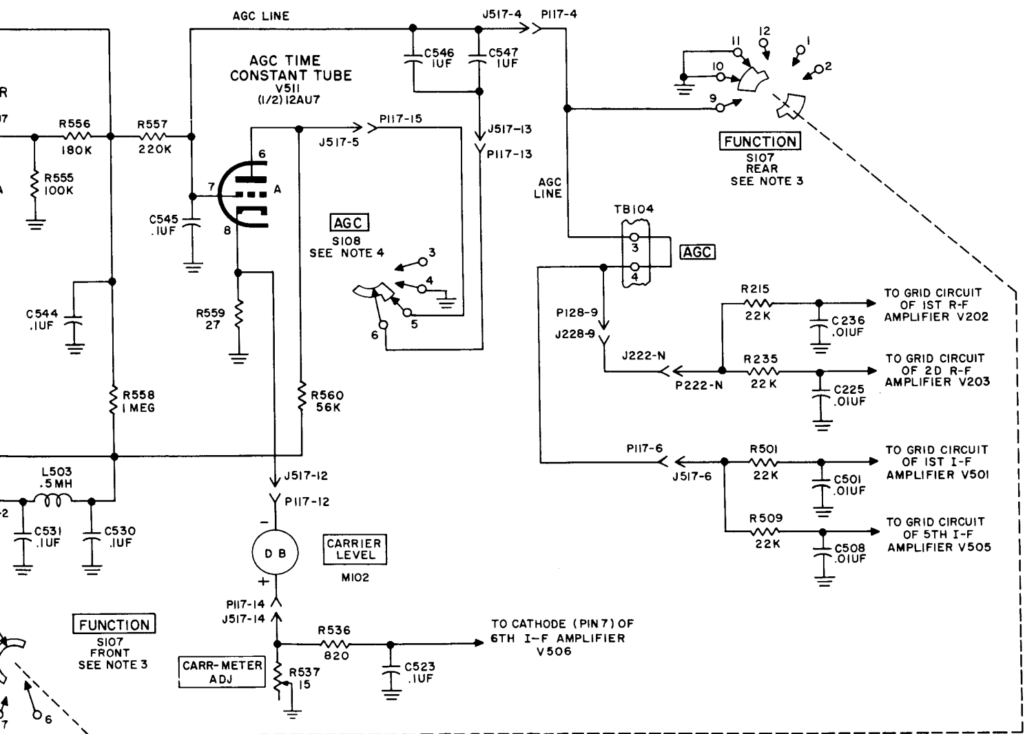
Figure 28. Agc circuit, schematic diagram.
