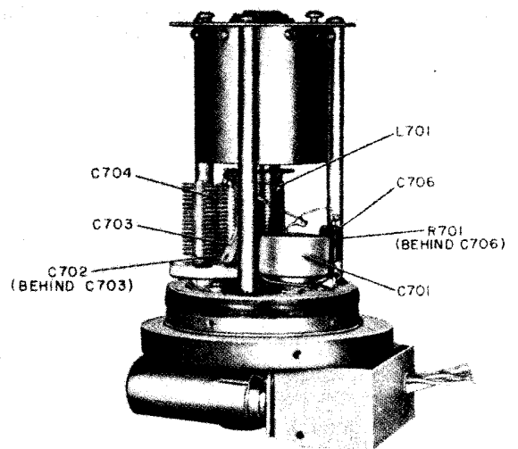
Figure 59. Vfo subchassis, cover and heating element removed.
