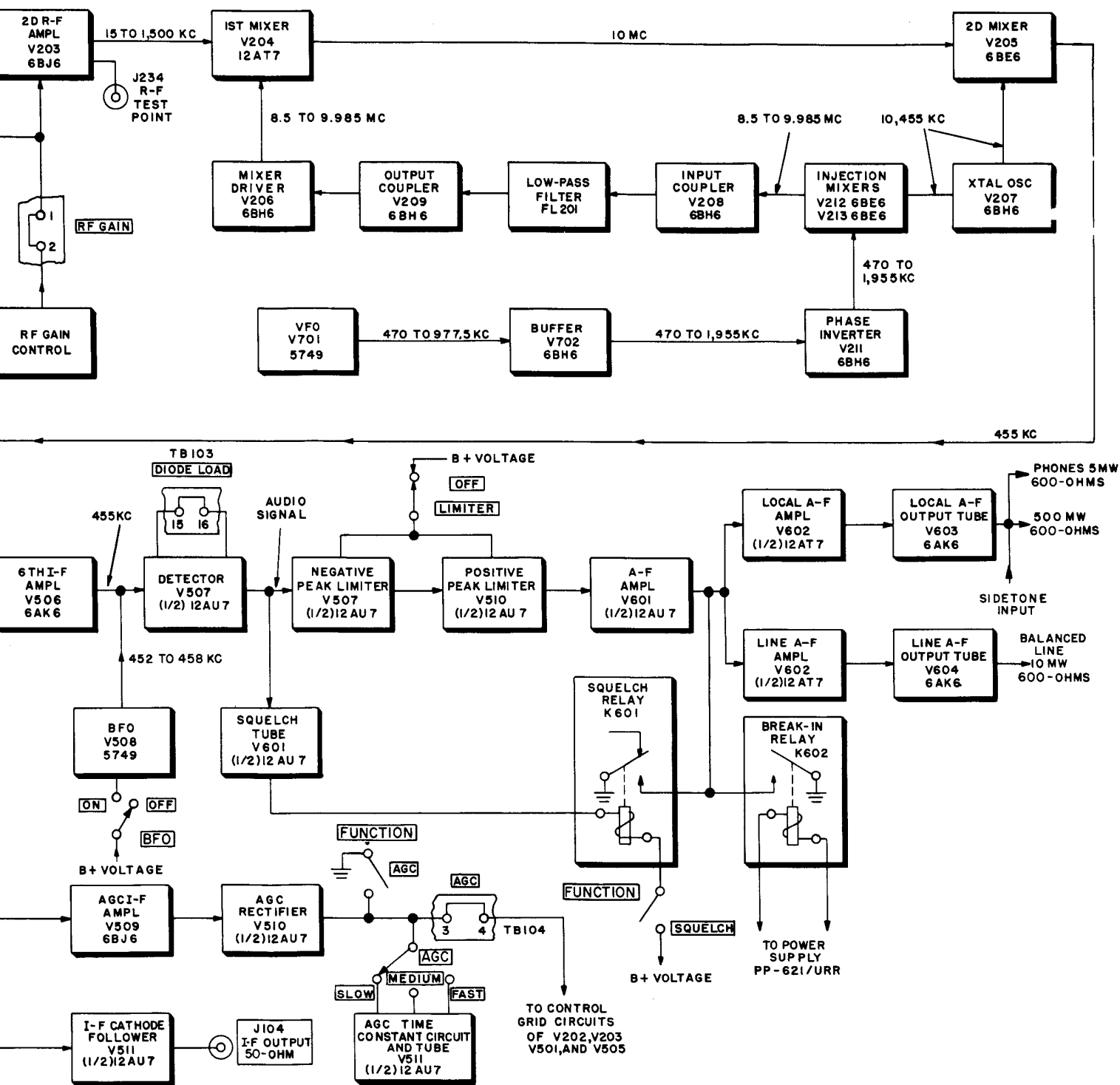
Receiver R-389/URR, block diagram.
