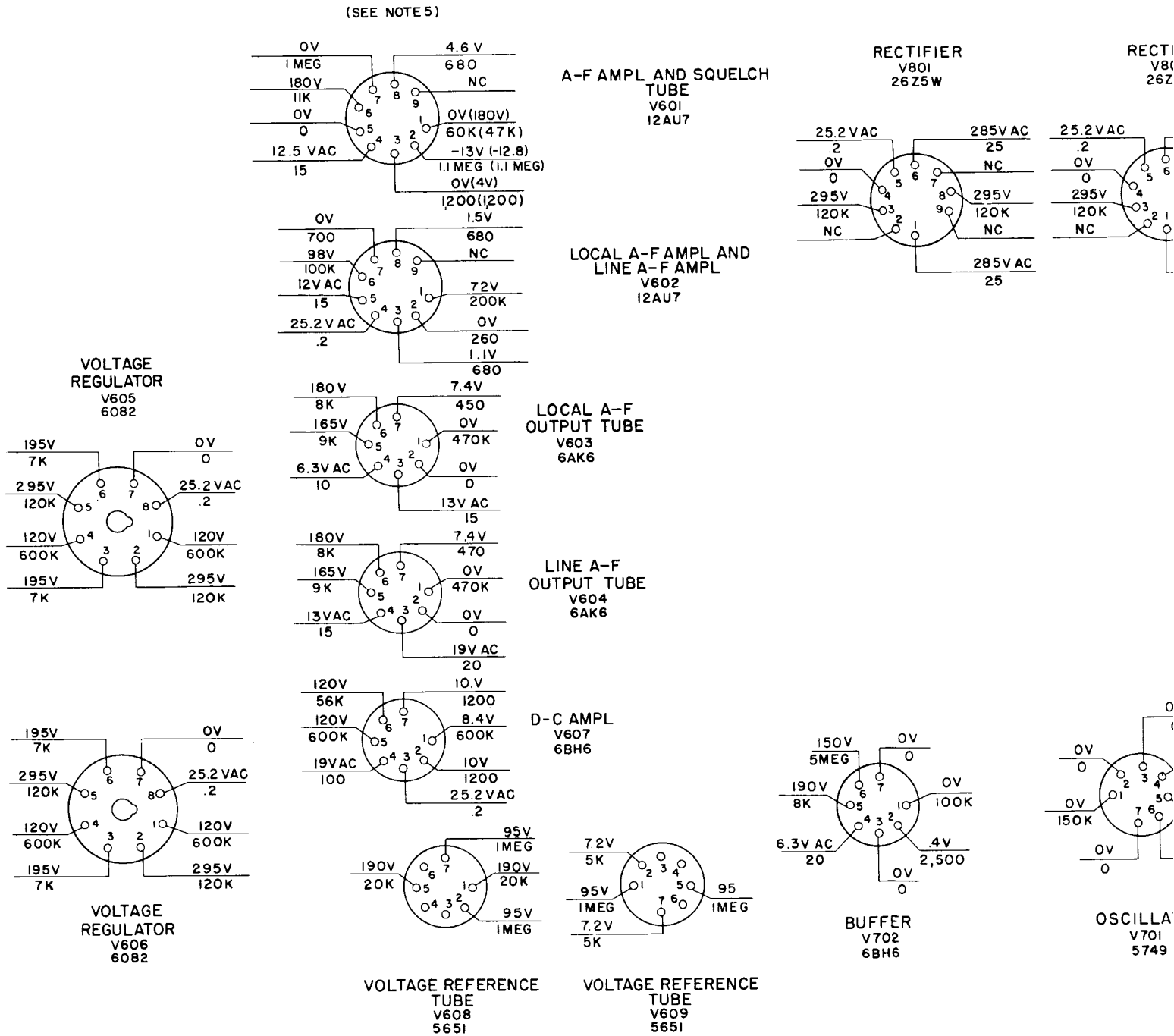
Figure 67. Tube-socket voltages and resistances
