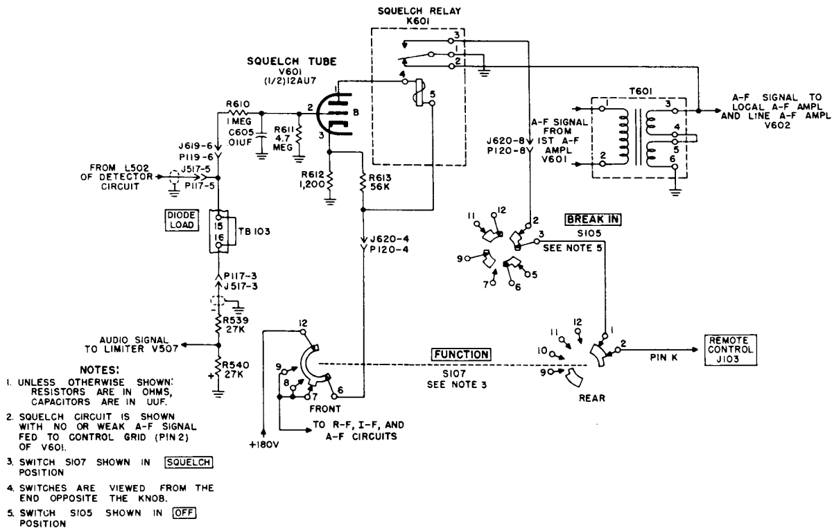
Figure 34. Squelch circuit, schematic diagram.
