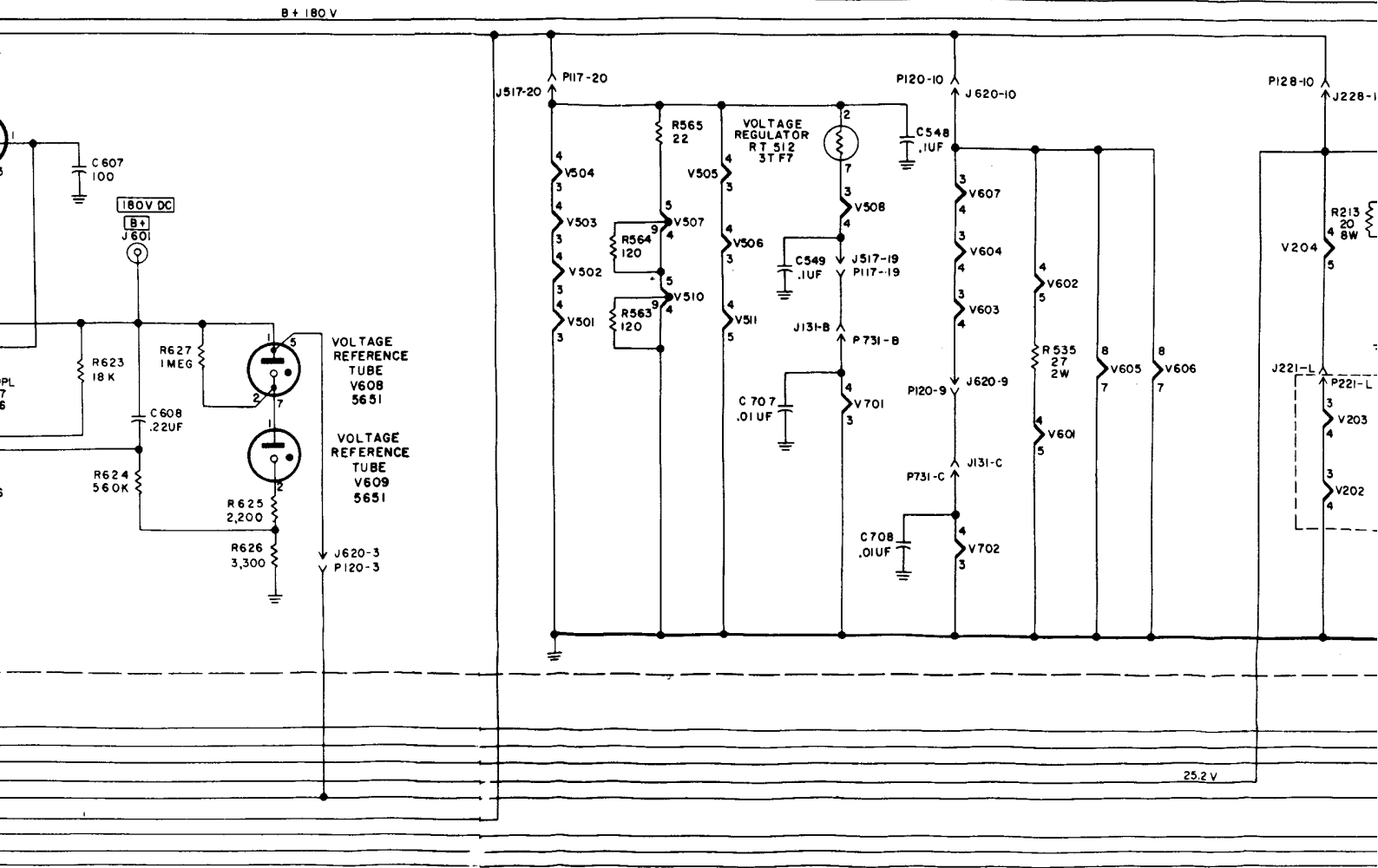
Figure 89. Radio Receiver R-389
