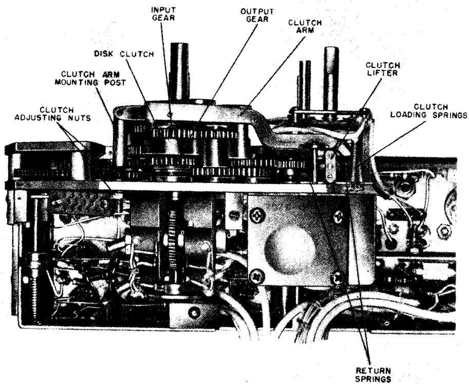
Figure 75. Disk clutch assembly, mounted.
