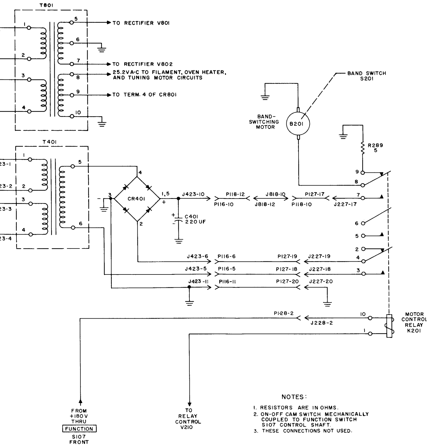
Band-switching motor power supply, schematic diagram.
