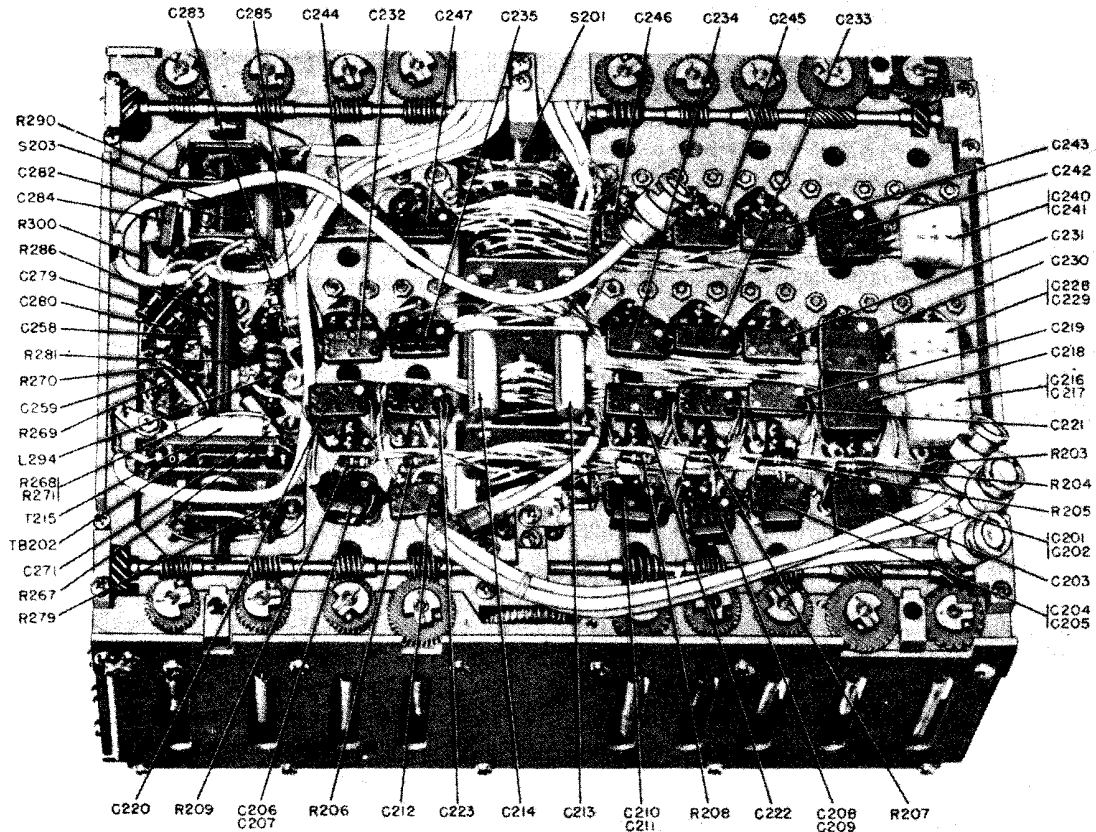
Figure 51. Rf subchassis, bottom view.
