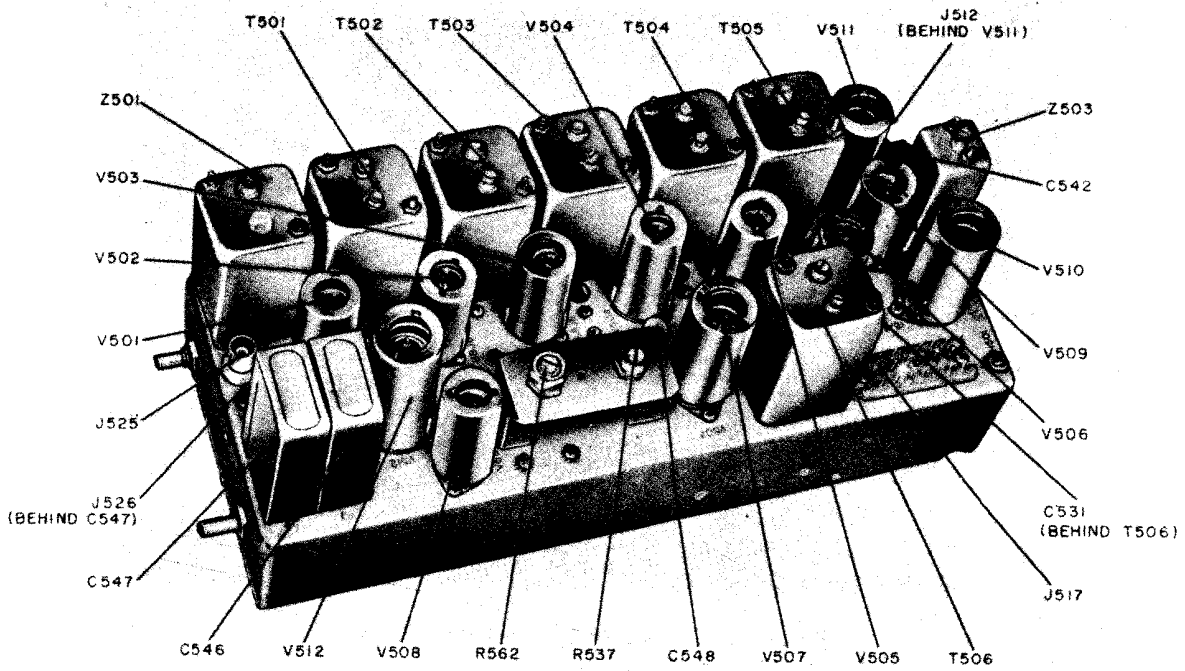
Figure 55. 1F subchassis, top view.
