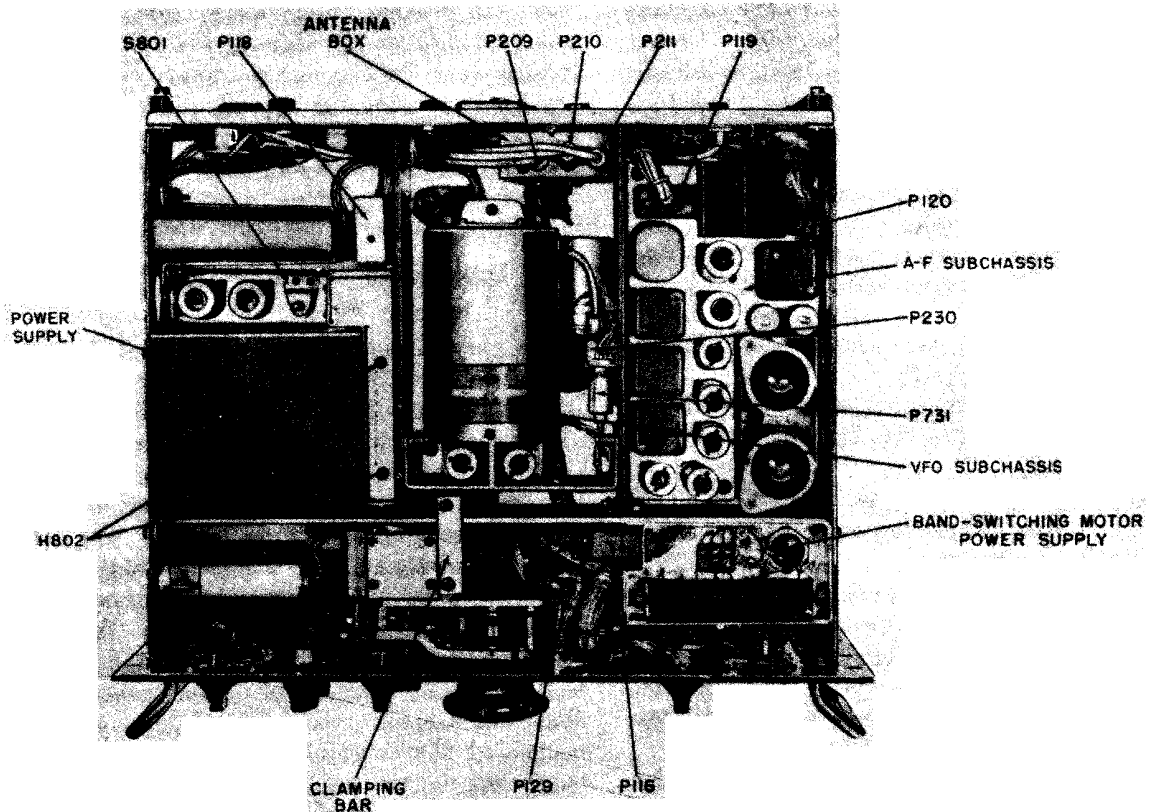
Figure 71. Bottom view, dust cover removed.
