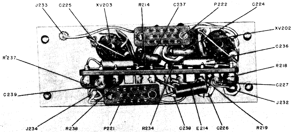
Figure 54. Rf amplifier, subassembly, bottom view.
