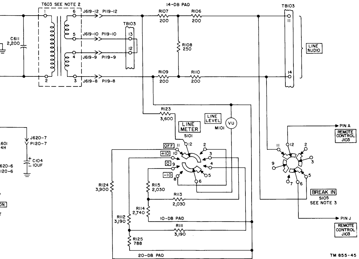
Figure 33. Line audio channel, schematic diagram.
