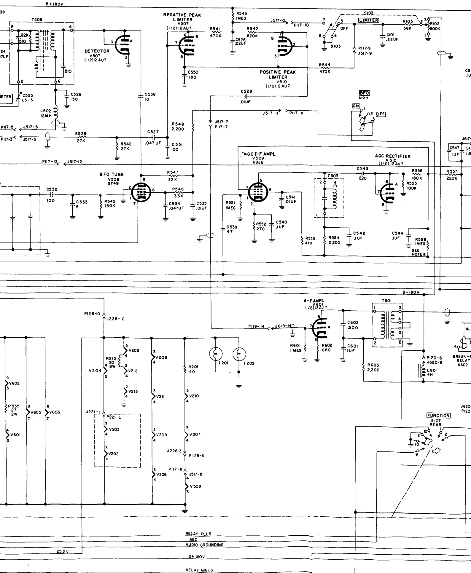
Figure 89. Radio Receiver R-389/URR, schematic diagram—Continued.
