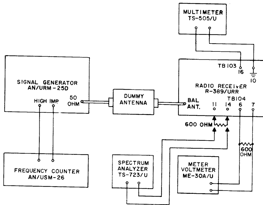
Figure 83. Equipment hookup diagram for testing Radio Receiver R-389/URR.
