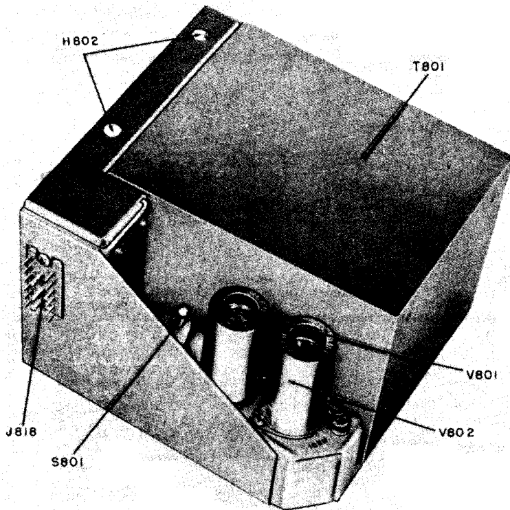
Figure 62. Power Supply PP-621/URR, top view.
