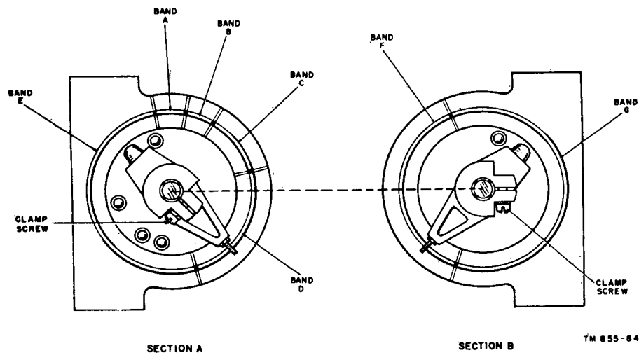
Figure 74. Band-switching motor control switch, showing segments and sliders.
