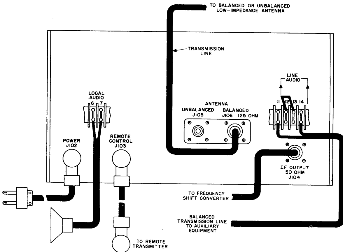
Figure 8. Cording diagram.
