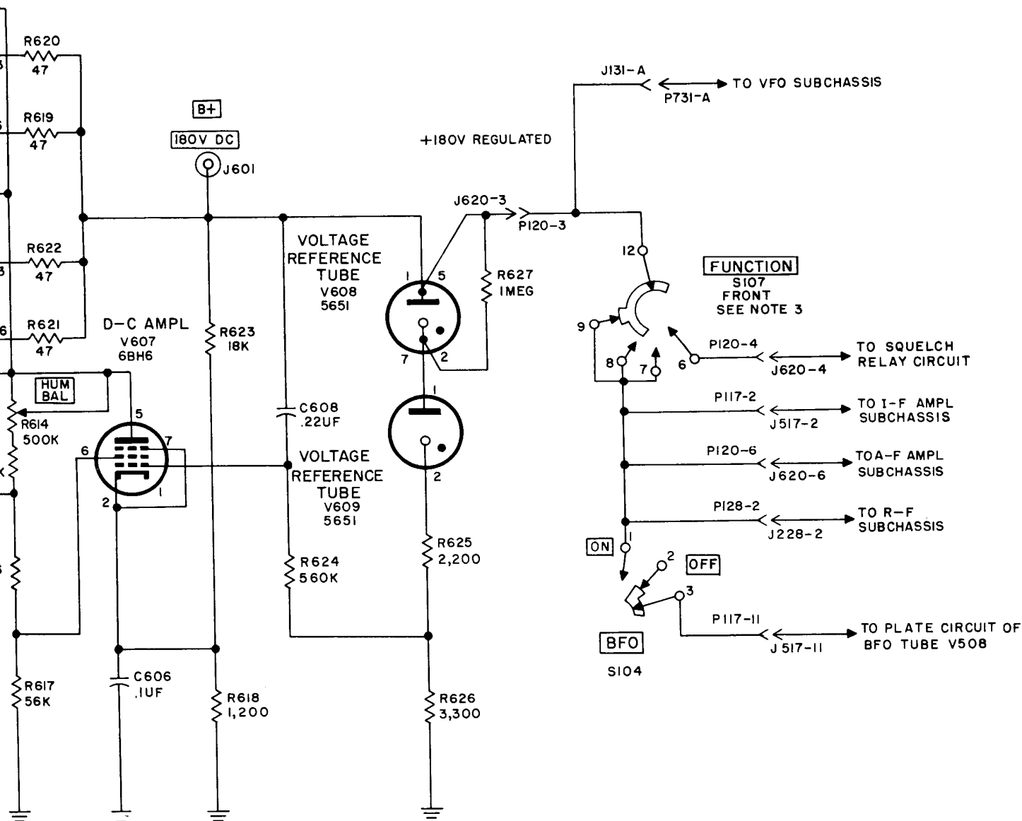
Figure 36. Voltage regulator, schematic diagram.
