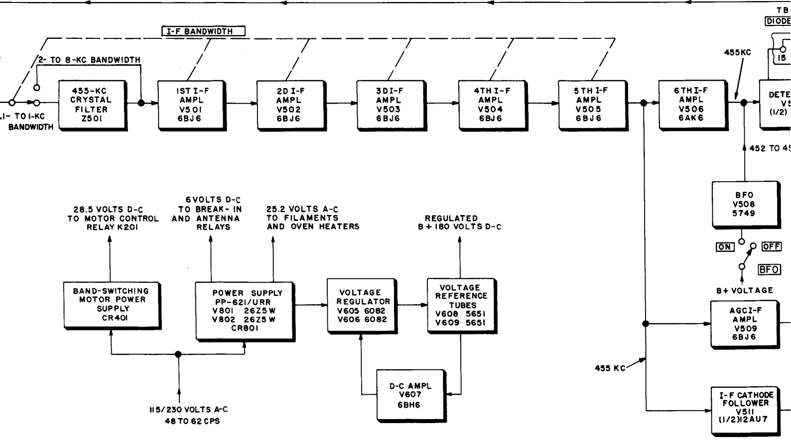
Figure 12. Radio Receiver R-389/URR, block diagram.
