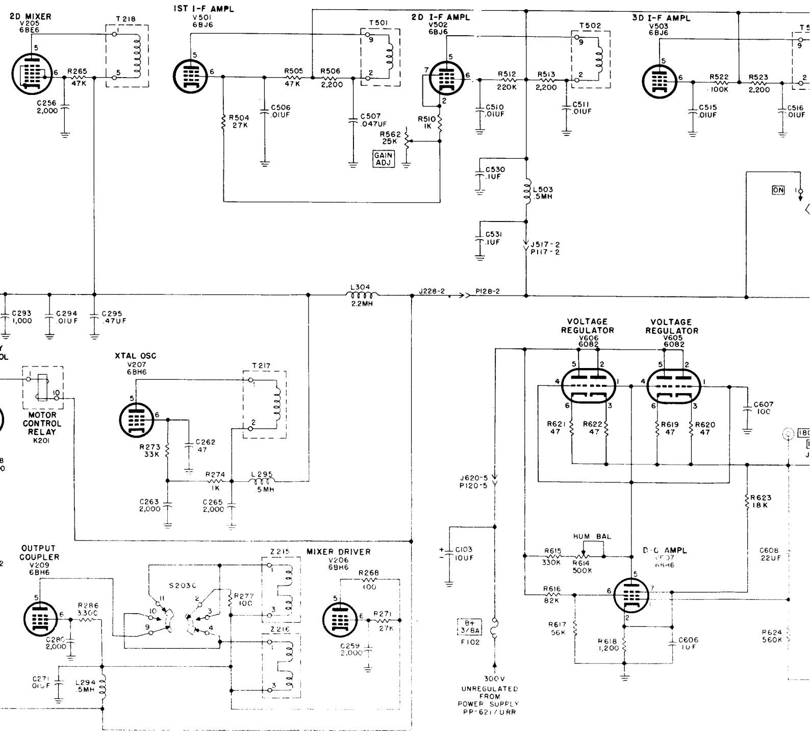
Figure 87. B+ voltage distribution.
