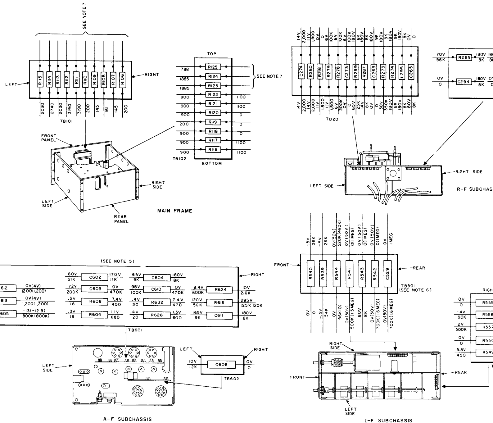
Figure 68. Voltages and resistances at terminal boards.
