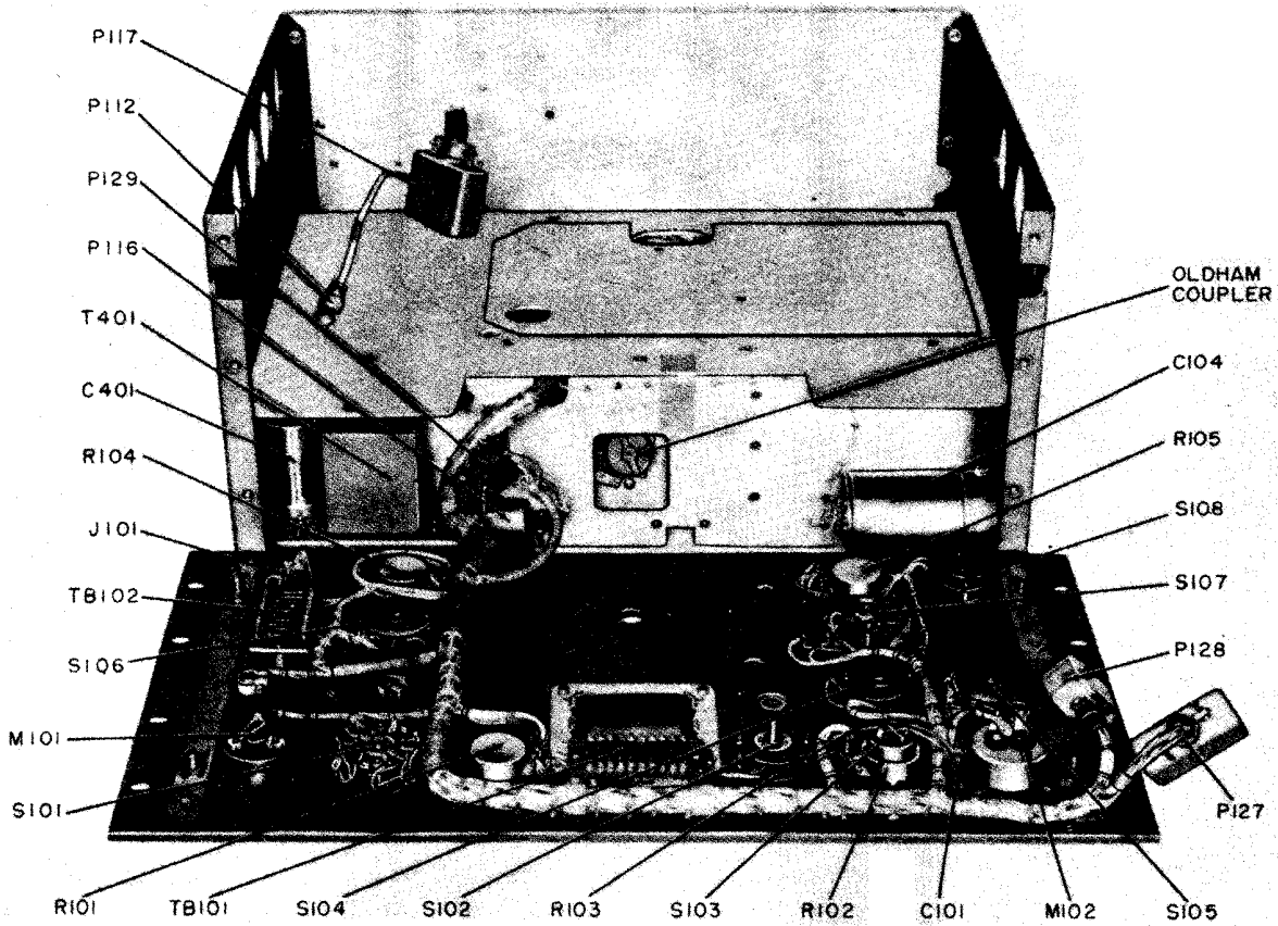
Figure 64. Front panel and main frame, top view.
