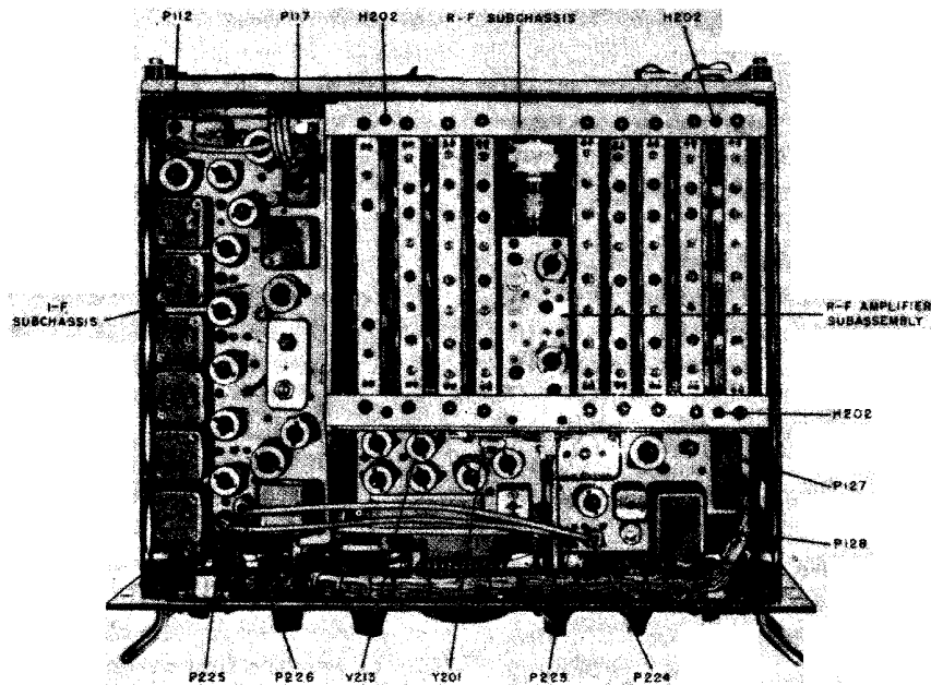
Figure 70. Top view, dust cover and shield removed.
