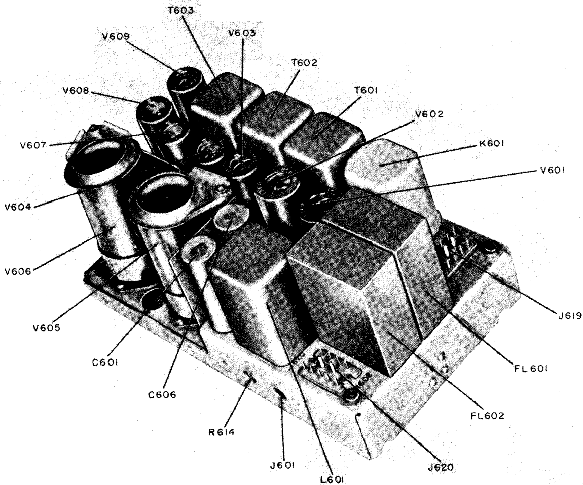
Figure 60. AF subchassis, top view.
