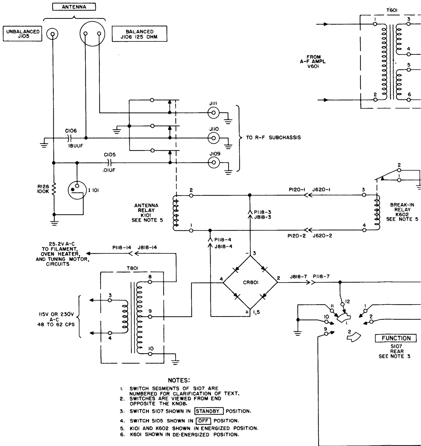
Figure 41. Break-in circuit
