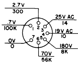
2D MIXER V205 6BE6
