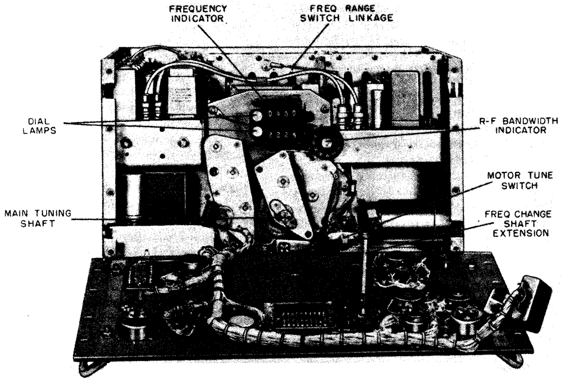
Figure 69. Front view, front panel removed.
