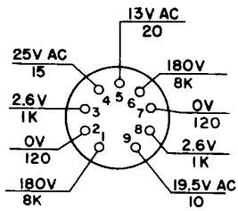
1ST MIXER V204 12AT7
