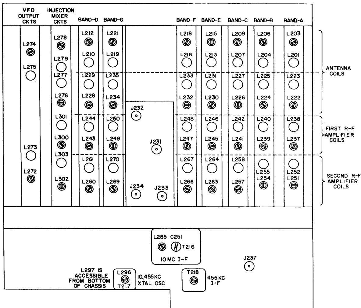
Figure 77. Location of rf alignment adjustments.
