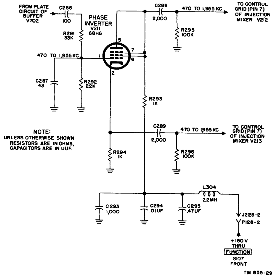
Figure 19. Phase inverter, schematic diagram.
