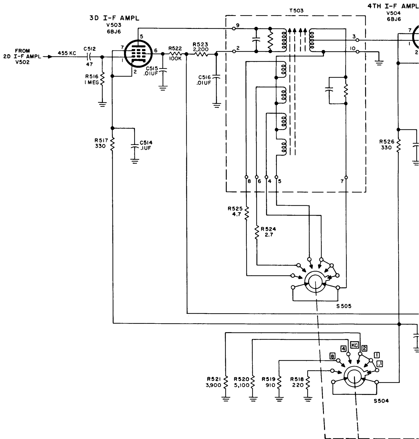
Figure 24. Third and fourth if. ampl
