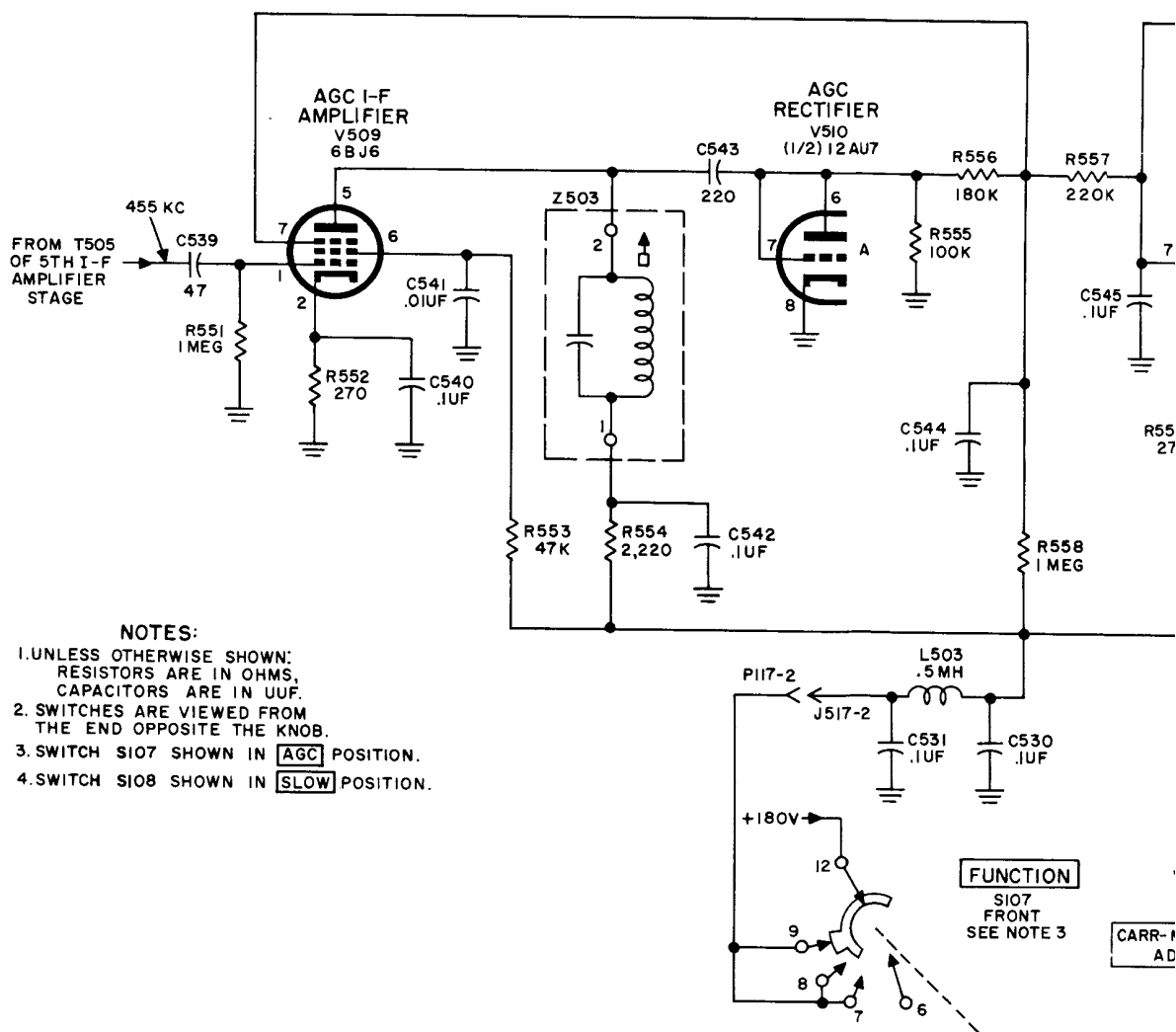
Figure 28. Agc circuit
