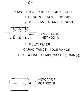
GLASS-DIELECTRIC, GLASS CASE
