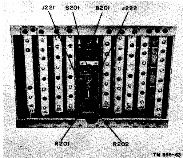
Figure 52. Section of rf subchassis, showing band-switching mechanism.
