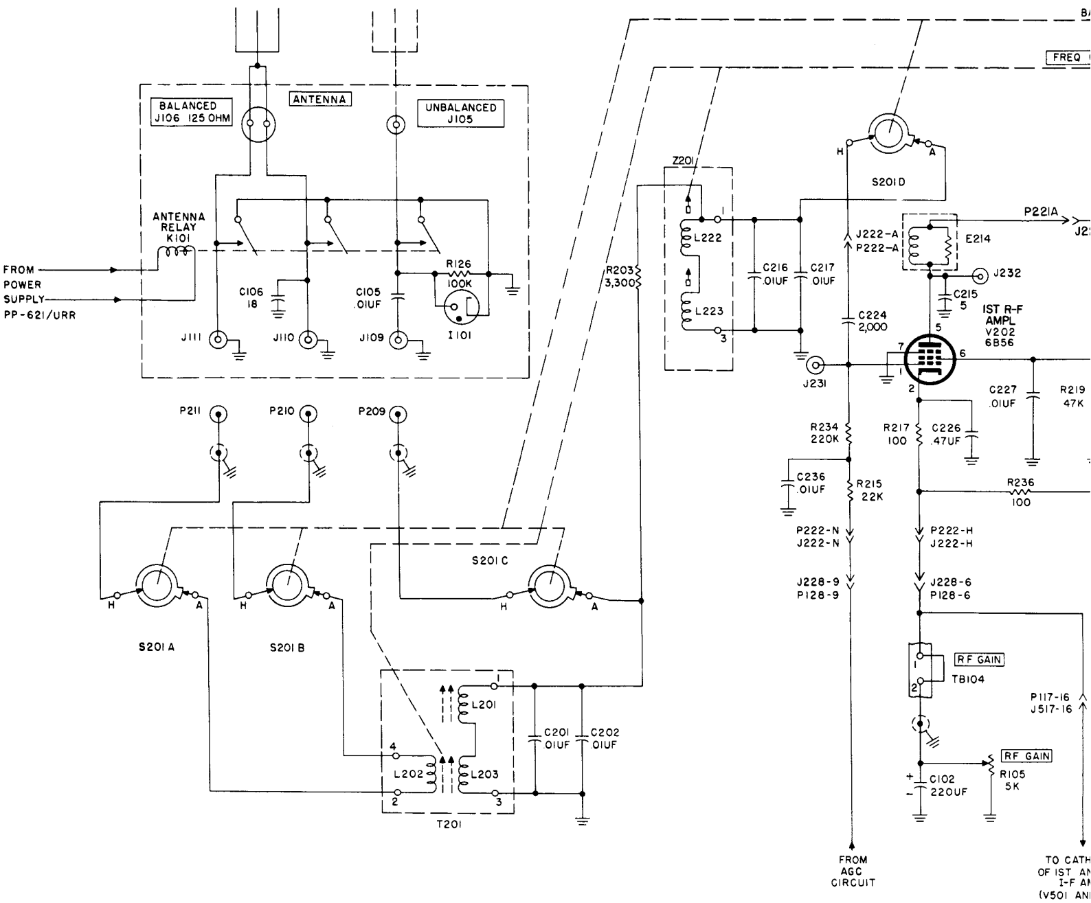
Figure 13. Antenna circuit and first rf amplifier, schematic diagram.
